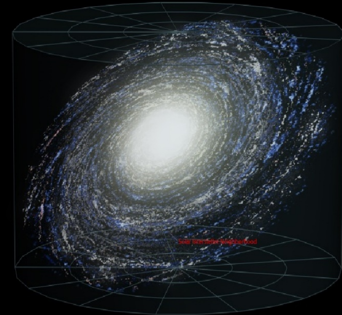
MILKY WAY GALAXY
