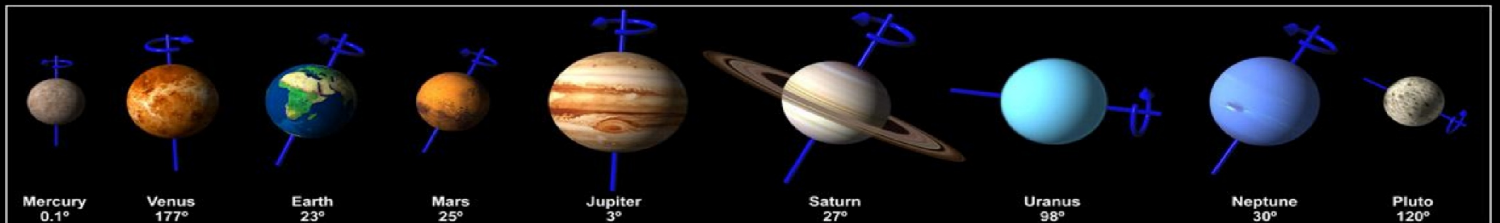
Obliquity of the Nine Planets
