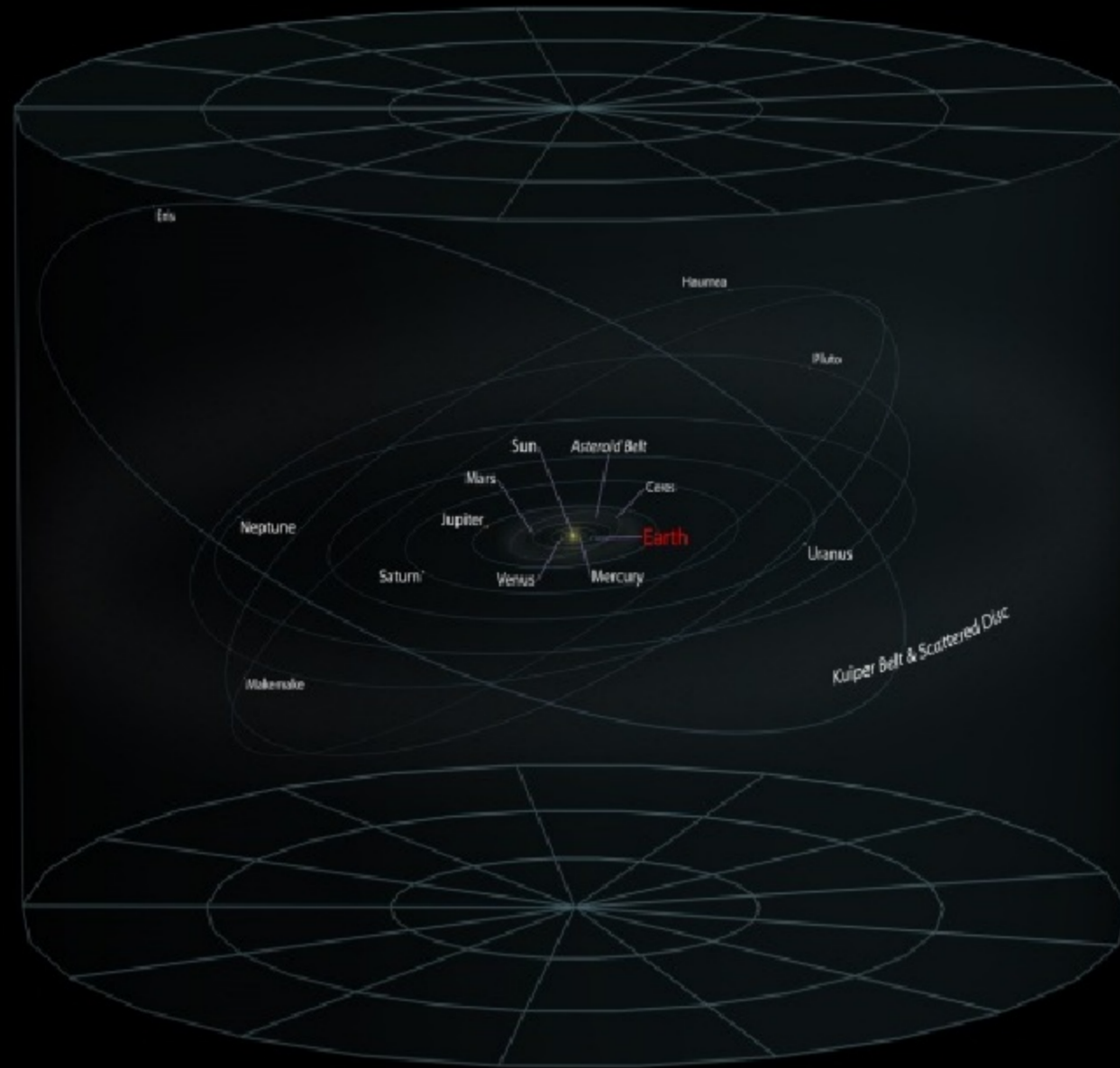
SOLAR SYSTEM
