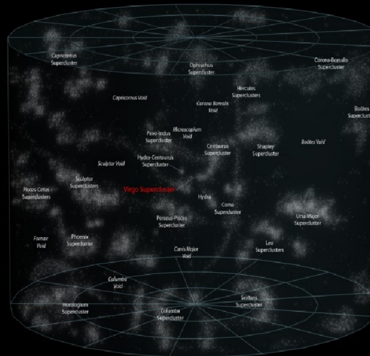
LOCAL SUPERCLUSTERS
