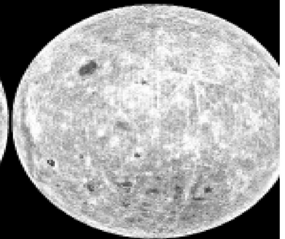
MOON'S "FAR" SIDE, HIDDEN FROM EARTH
