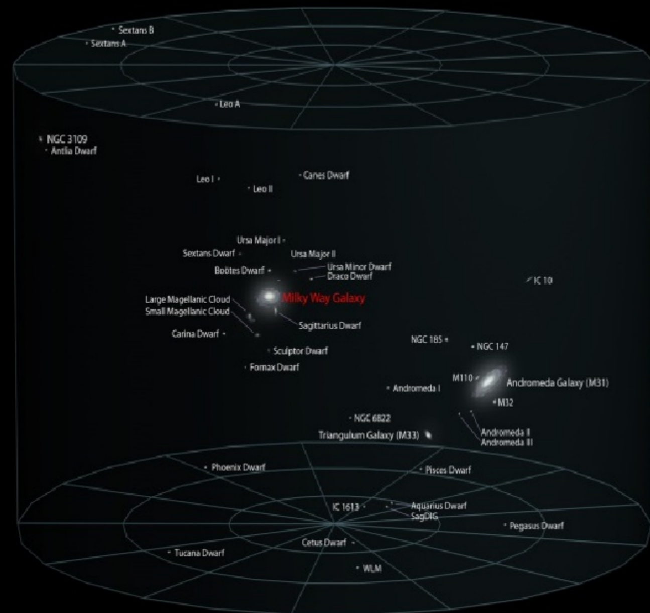
LOCAL GALACTIC GROUP
