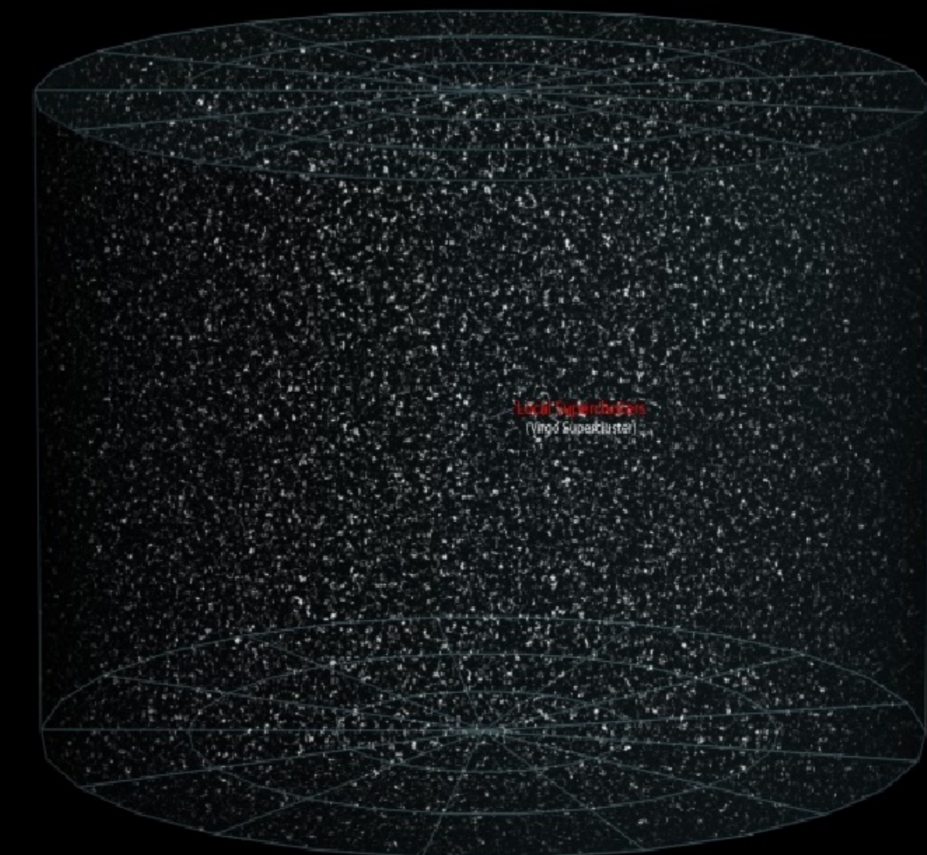
OBSERVABLE UNIVERSE
