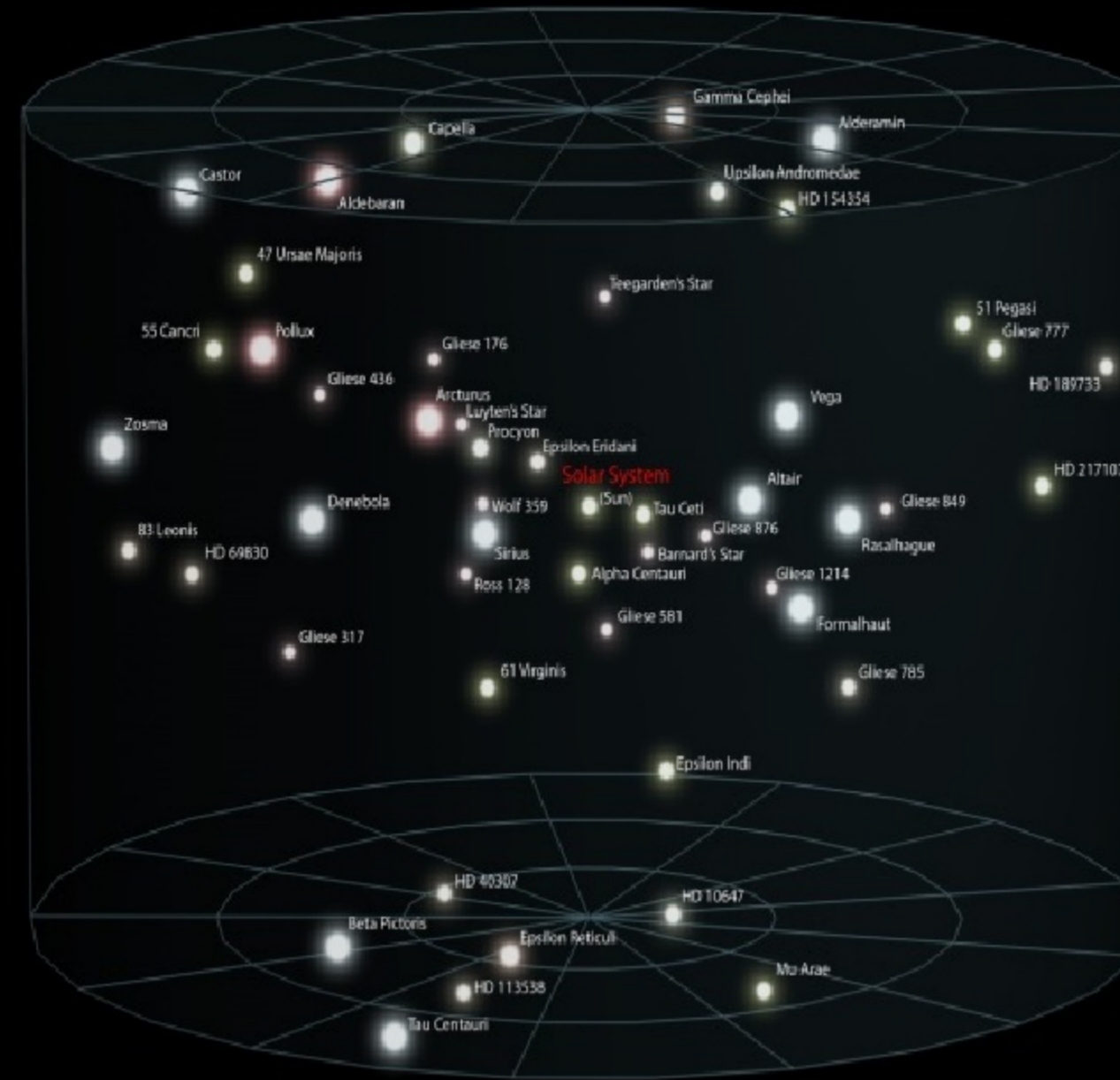
INTERSTELLAR NEIGHBORHOOD
