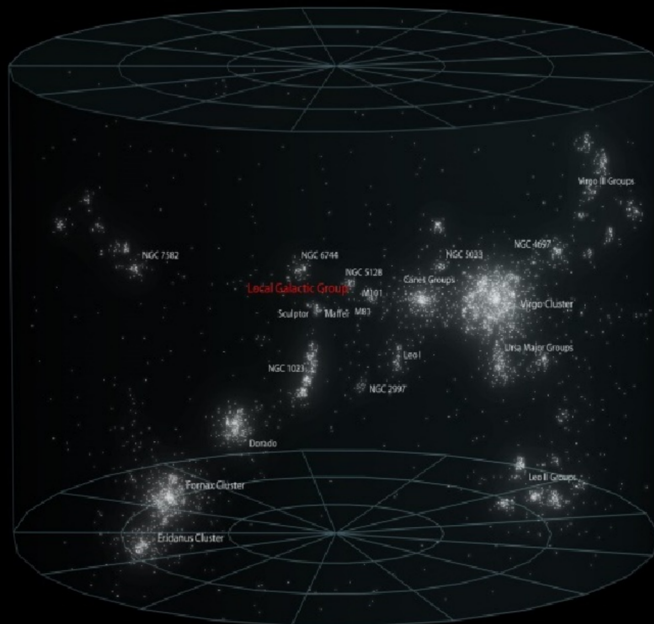
VIRGO SUPERCLUSTER
